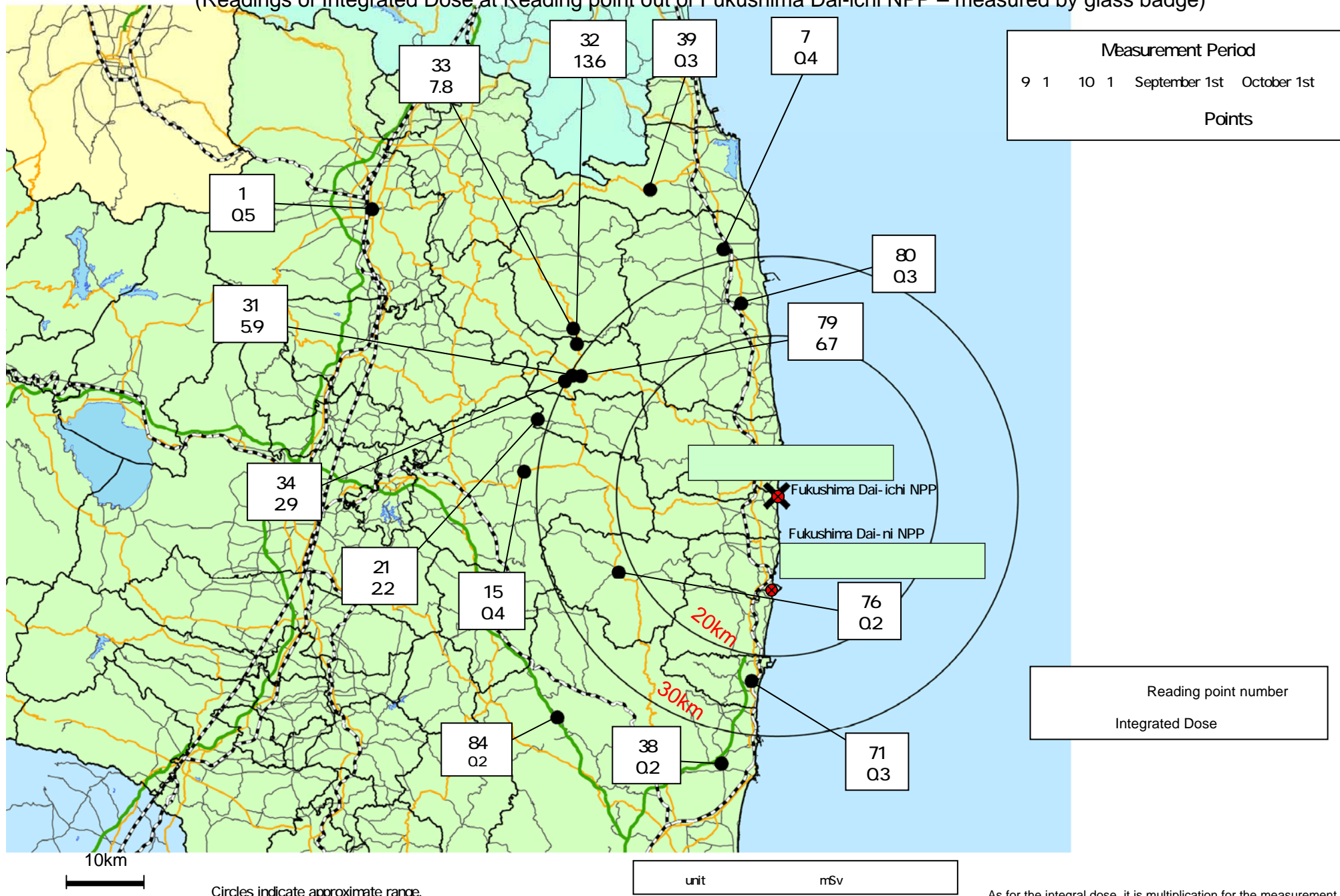
(Readings of Integrated Dose at Reading point out of Fukushima Dai-ichi NPP – measured by glass badge)
